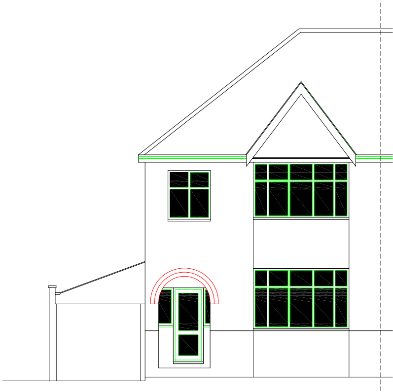
EXISTING FRONT ELEVATION 1:100 @ A3
